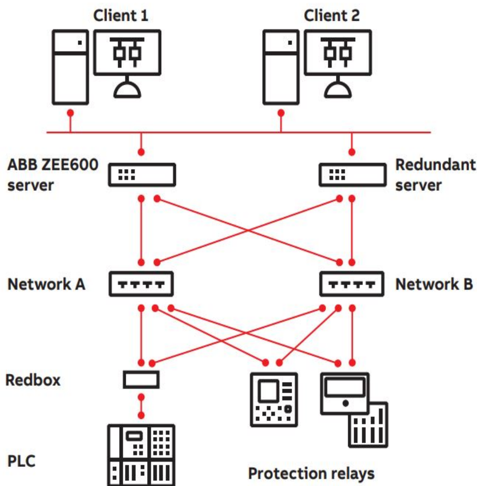
Figure 44. ZEE600 communication redundancy
