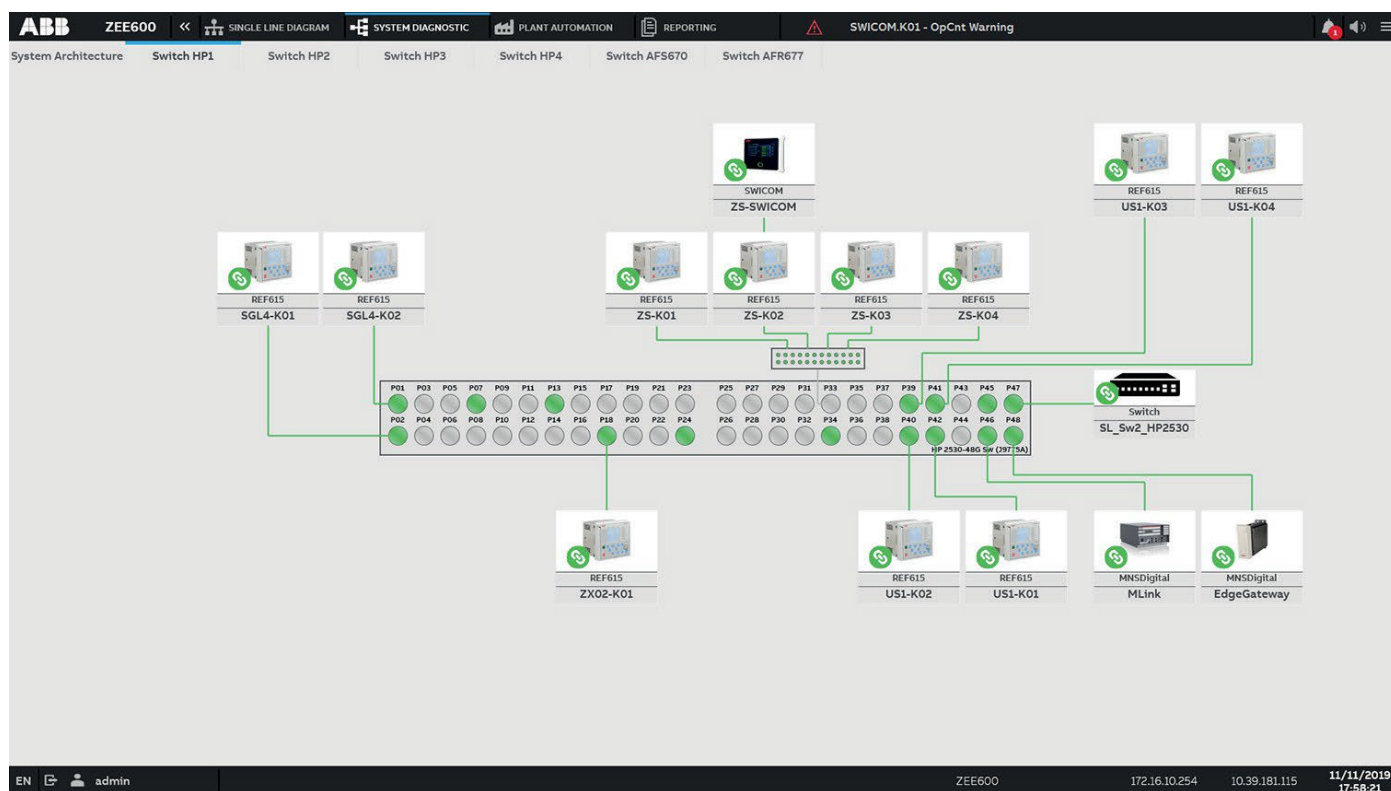
Figure 11. ZEE600 connectivity states
