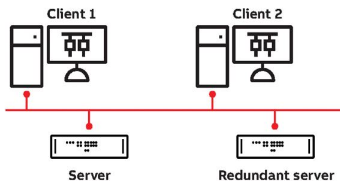
Figure 41. ZEE600 client-server
