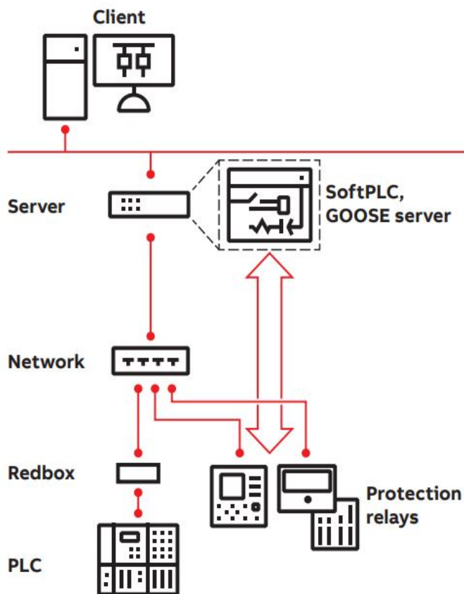
Figure 47. ZEE600 IEC 61850 GOOSE supervision
