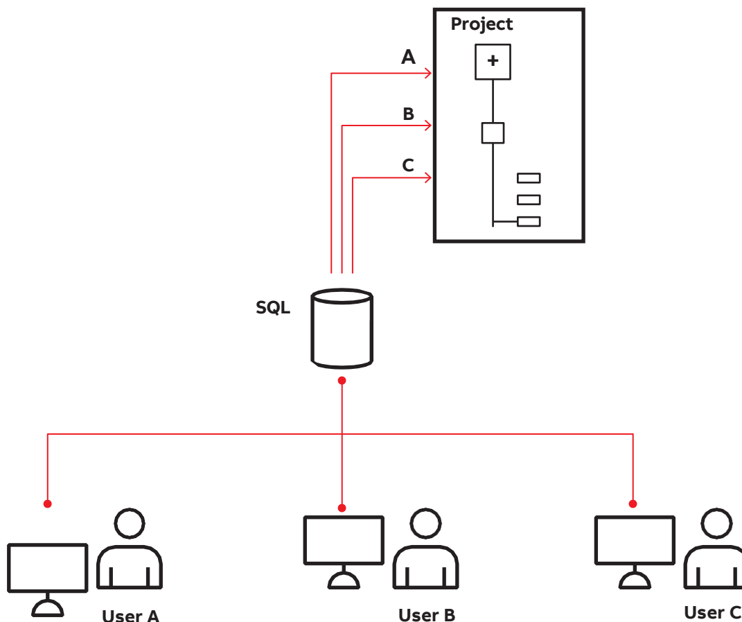
Figure 48. ZEE600 distributed engineering
