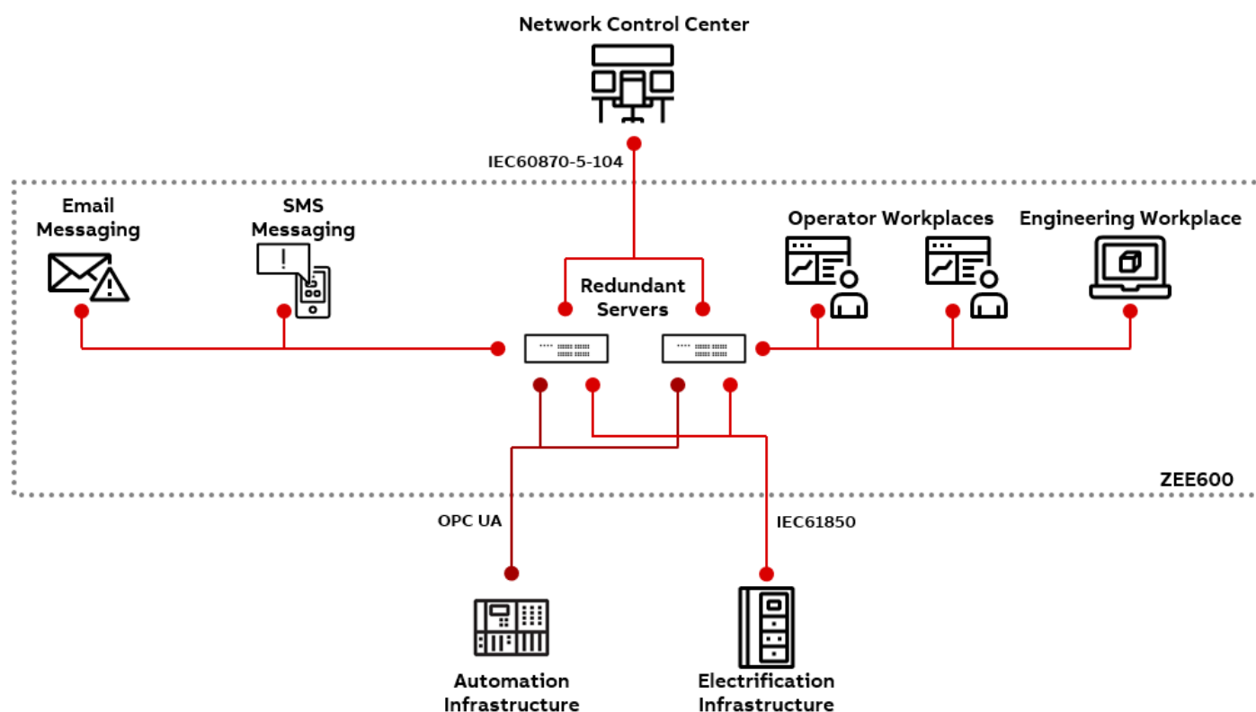
Figure 52. System drawing
