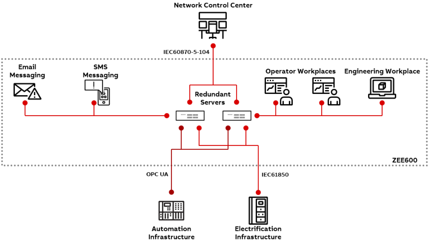
Figure 50. Example System Drawing
